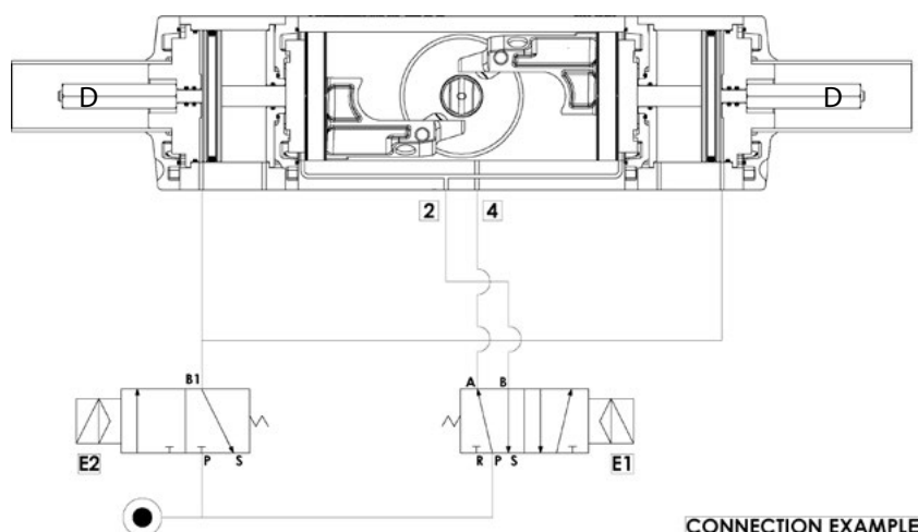
CONNECTION EXAMPLE
